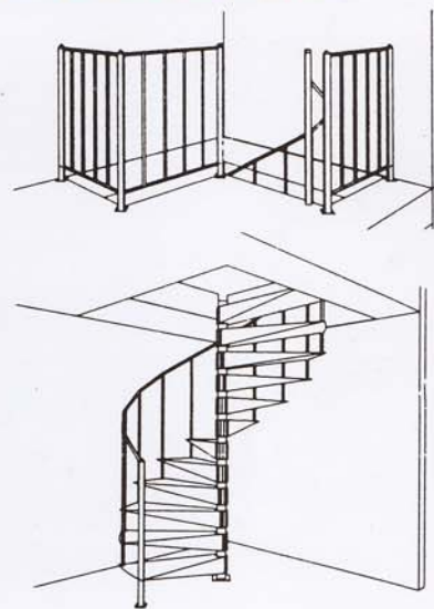
S Model
